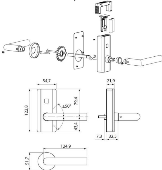
Okucie C-lever-compact K6
